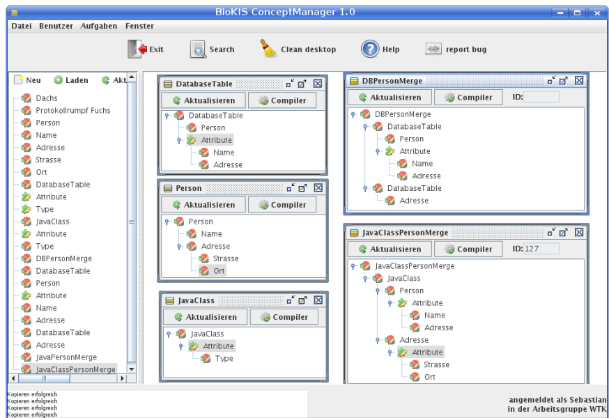
Abbildung 1: ConceptManger for Supporting Concept-Driven Engineering
